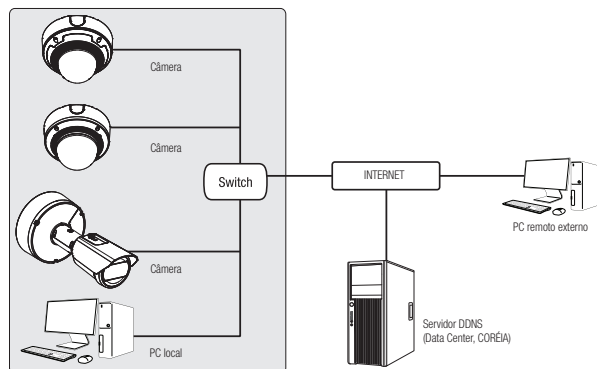
<Rede local>
