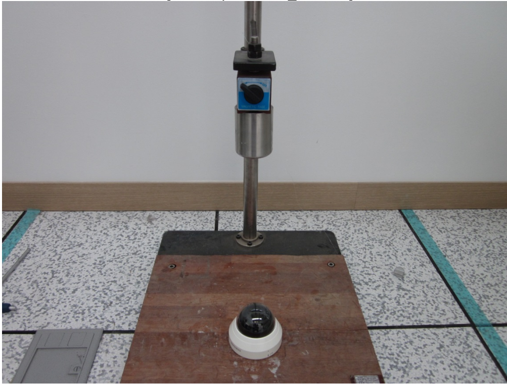
[IK08 Impacts Test_Window]
