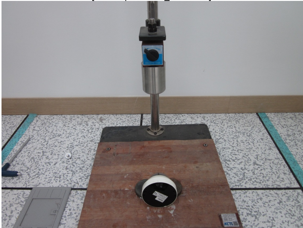
[IK08 Impacts Test_Enclosure]
