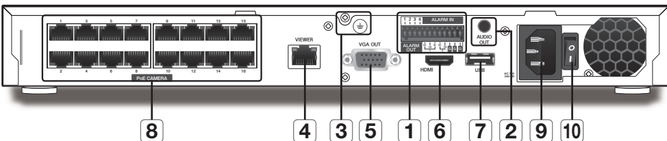
QRN-1610S
