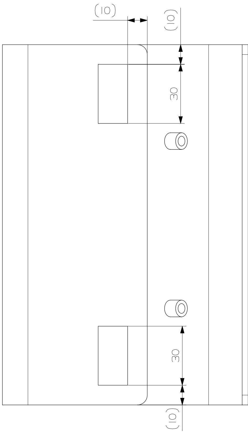
VIEW A
