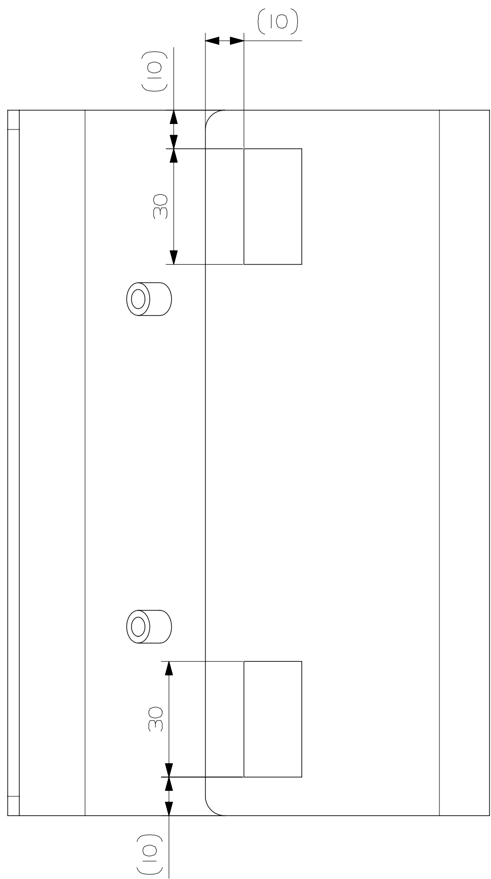
VIEW B
