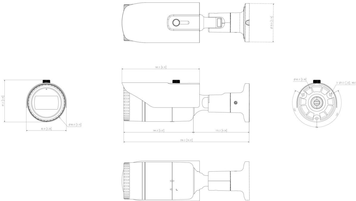
Apperance SCO-6085R, SCO-6085RVP, SUO-6085R UNIT : mm[inch]
