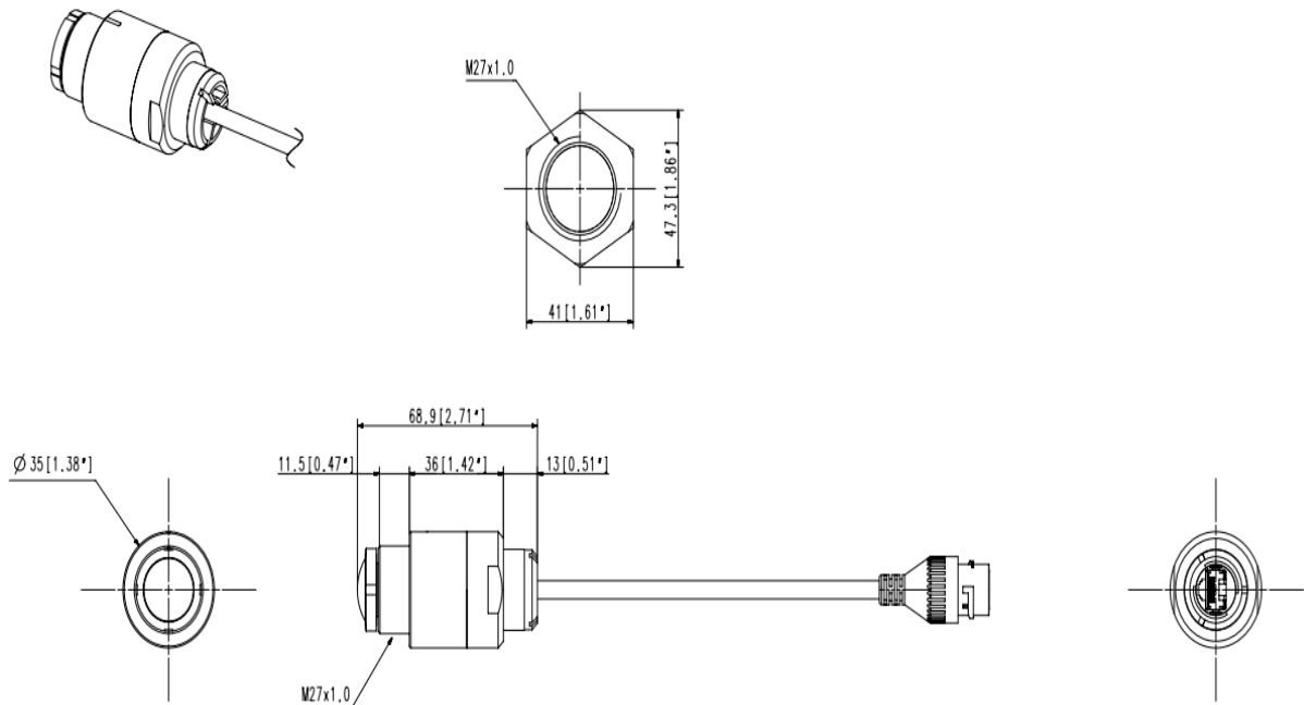
Construction Diagram
