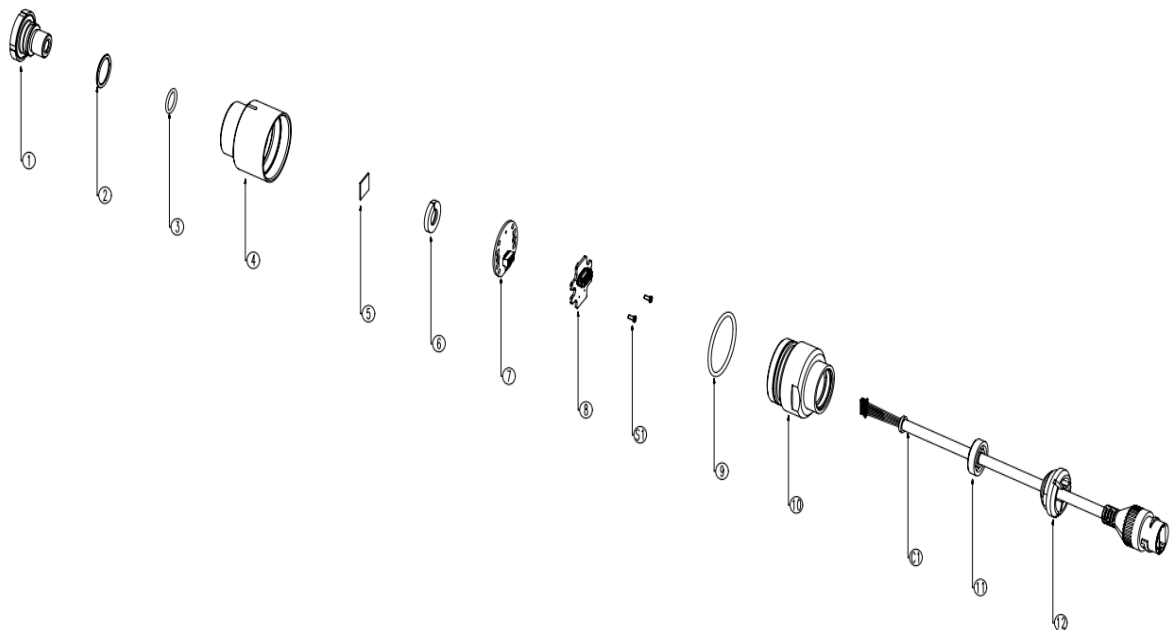
Installation method
