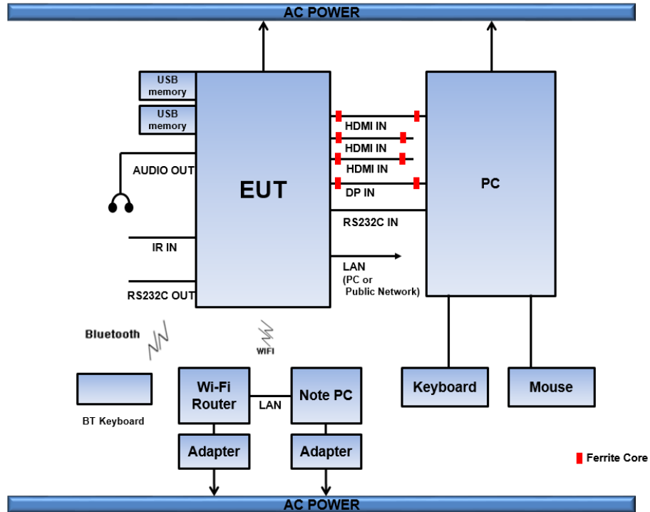
[Operating mode 1, 2]
