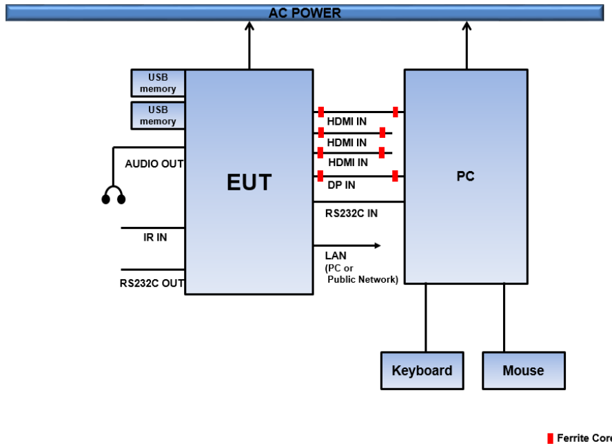
[Operating mode 3, 4, 5]
