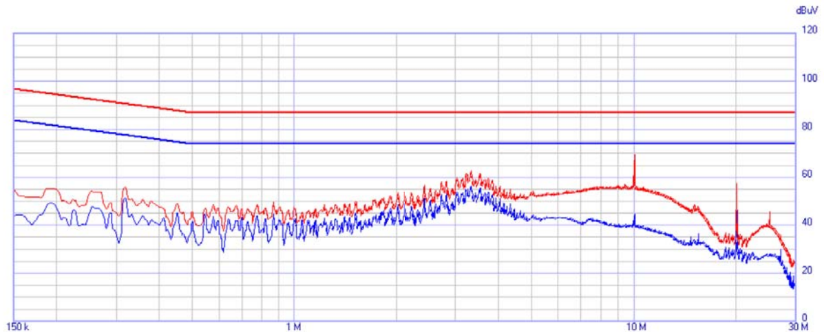
SNB-6011P_TEL 10 Mbps_AC-DC Adapter
