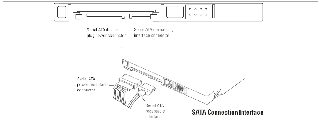
Figure 5-1. Connector Locations
