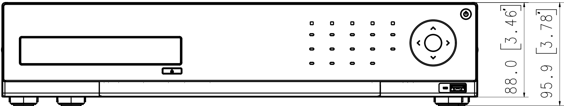
Appearance SRS-1676D Unit : mm[inches]
