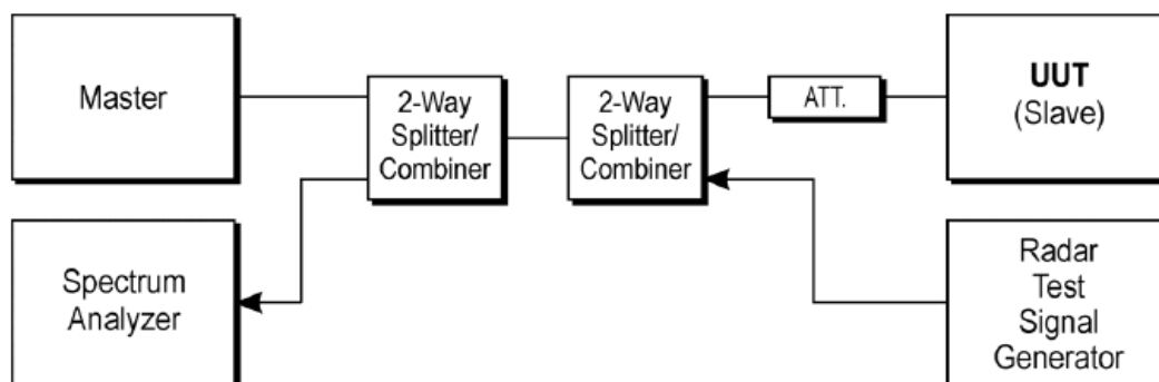
Figure 5: Set-up B
