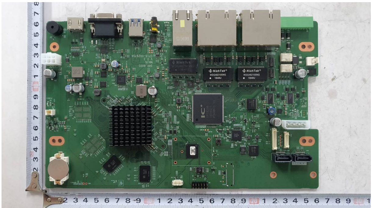
<Photo 8 > Main board _ Top view
