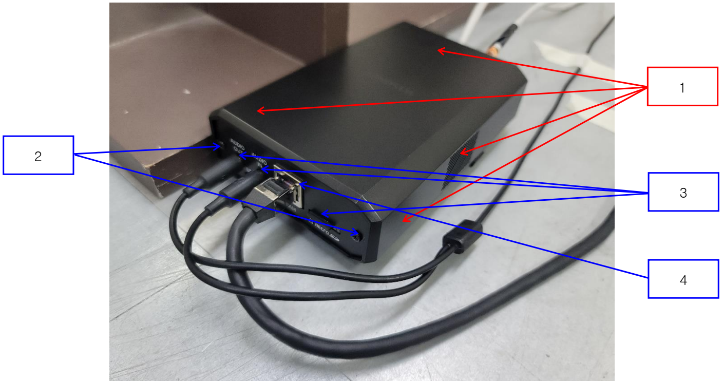
[시험기자재]-PoE
