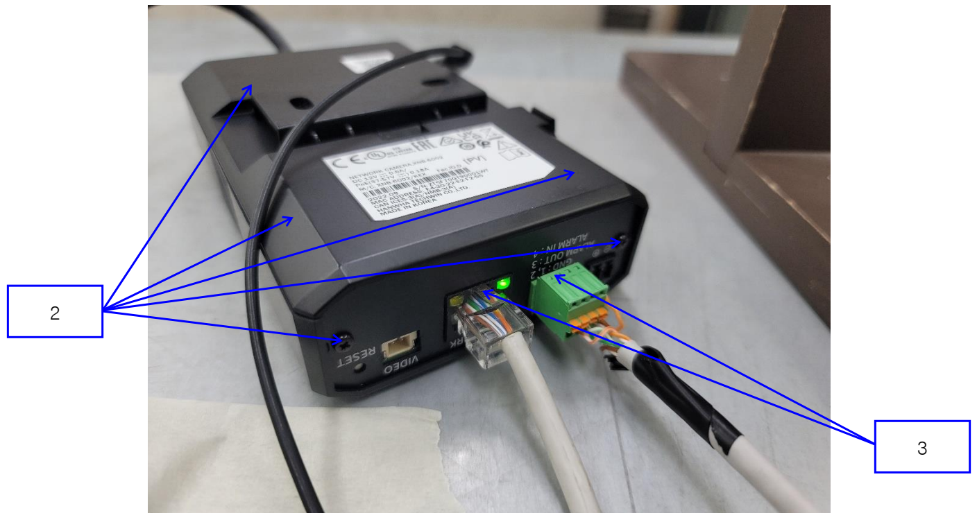
[시험기자재]-PoE
