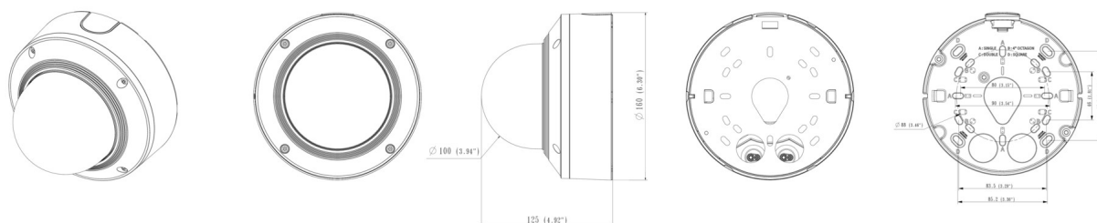
XND-6081VZ/8081VZ with SKIN-COVER
