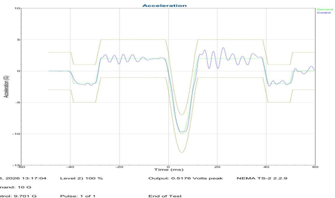
Mechanical Chock data -X Axis
