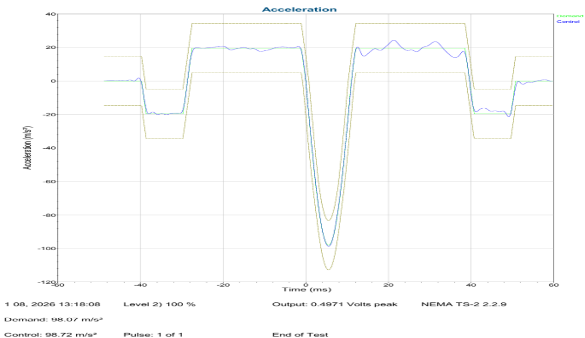
Mechanical shock data -X Axis
