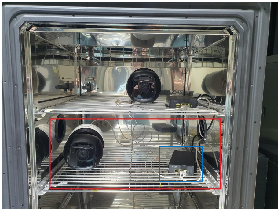
[Red square, test sample, blue square PoE Injector]
