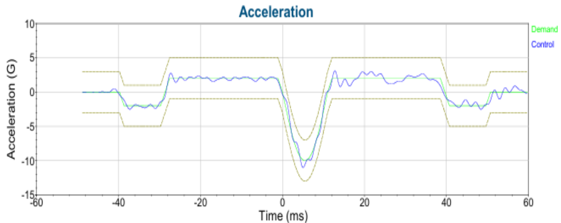
Mechanical Chock data +X Axis
