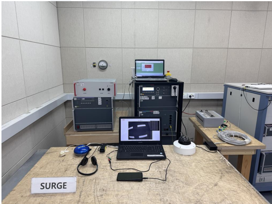
<Surge> Mode 1
