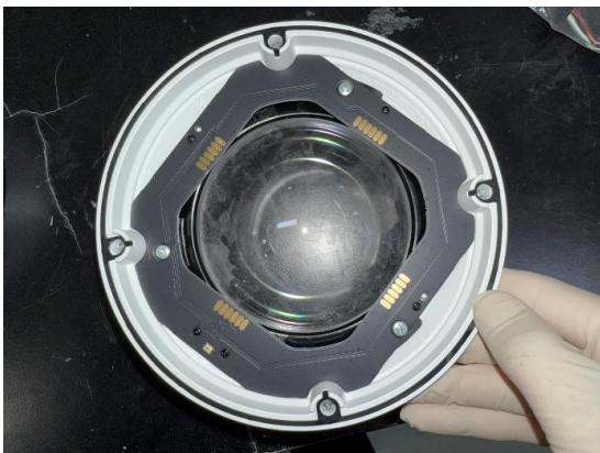
Figure 23) Photo after the test (Inside #2, Enlarge)
