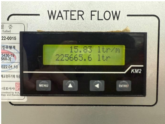
Figure 16) Photo of test condition (flow rate)
