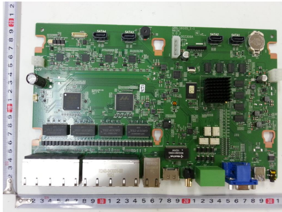
<Photo 9 > Component side – Main Bd.
