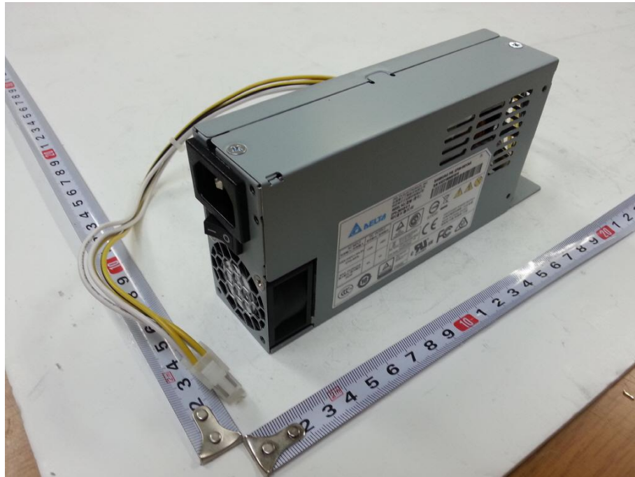
<Photo 11 > Front side – SMPS
