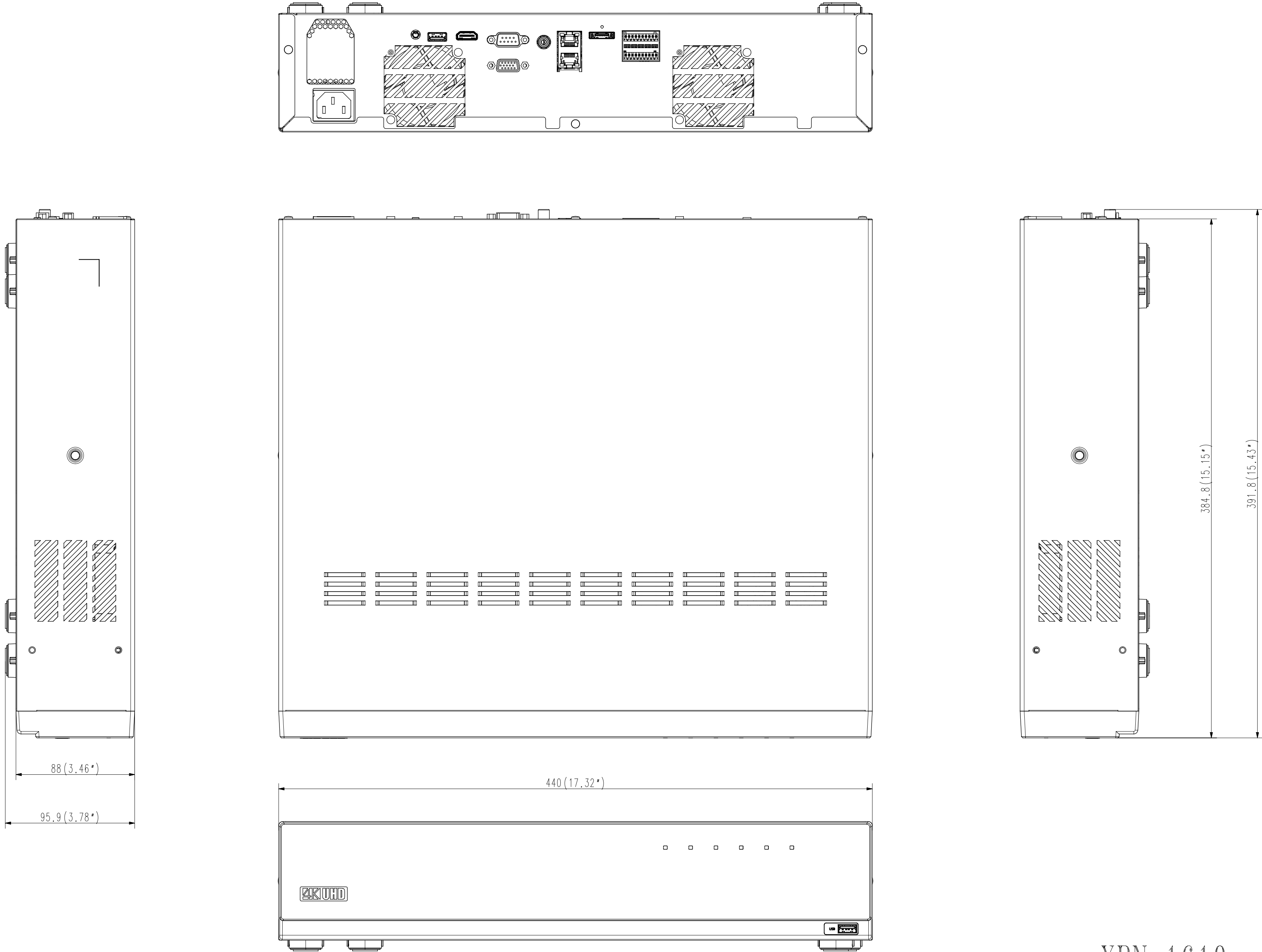
XRN-1610 Appearance drawing
