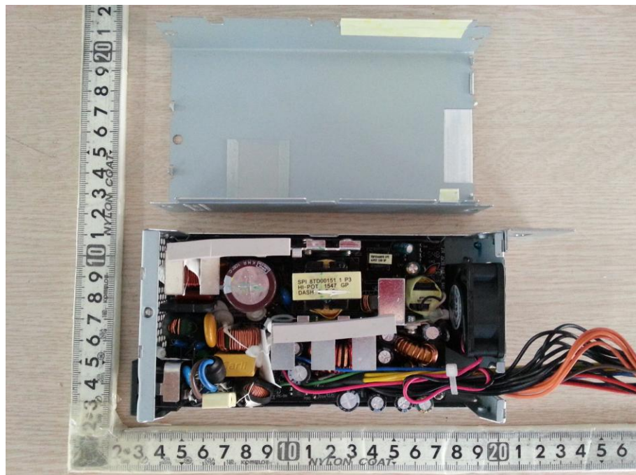
&lt;Photo 17 &gt; Inside – SMPS
