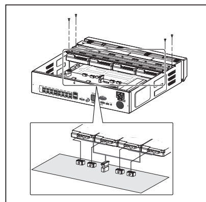
<XRN-1610S/1610SA>
