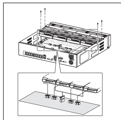
<XRN-1610S/1610SA>
