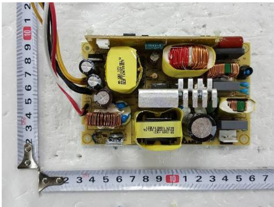
<Photo 12> SMPS view 3
