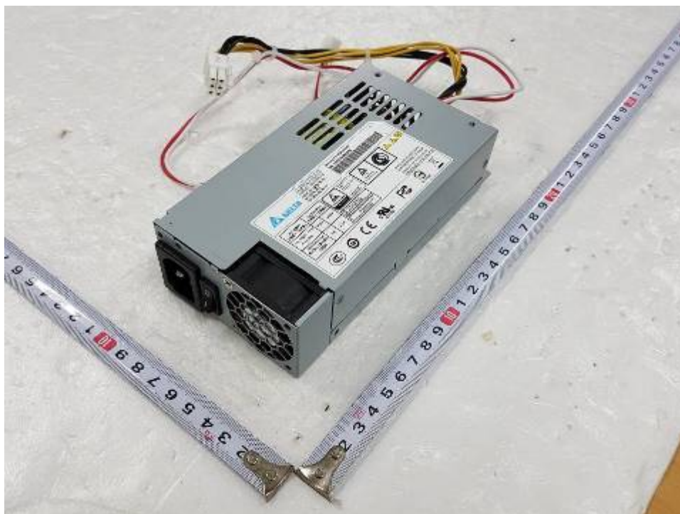
<Photo 10> SMPS view 1
