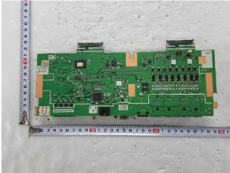
<Photo 8> USB board – top side
